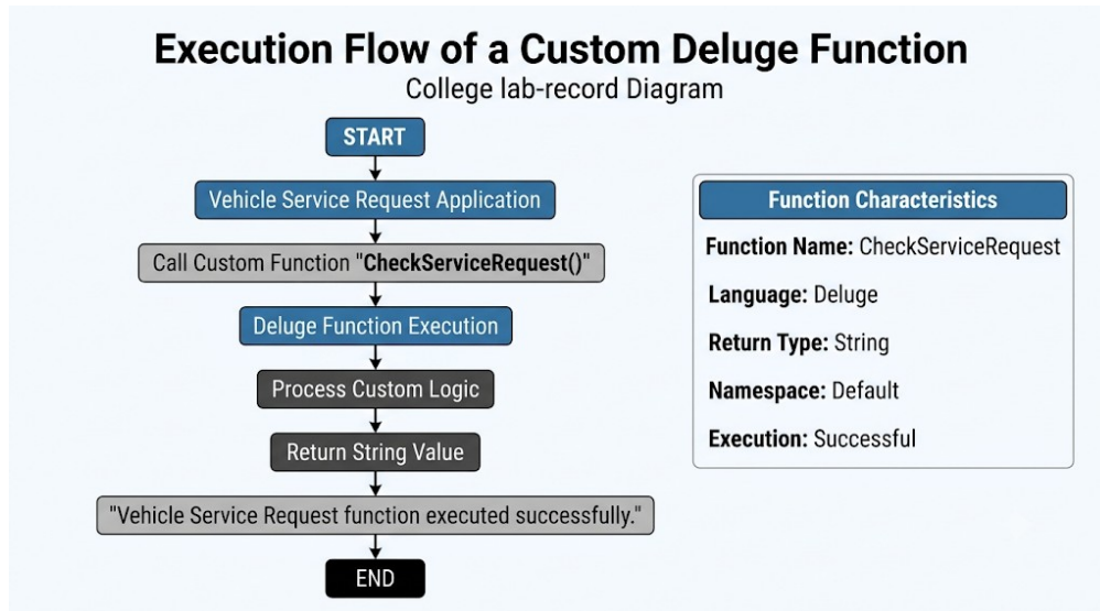
Figure 7: Execution Flow of a Custom Deluge Function (Supporting Diagram)
